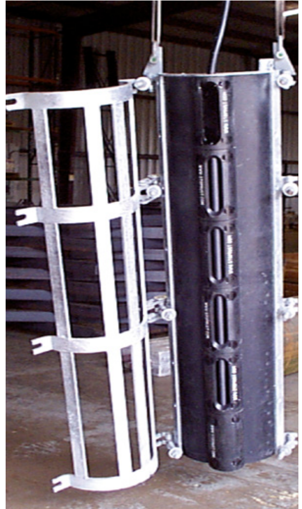
RAPAROUND 24" hinged 50-ampere harsh-environment anode assembly.
