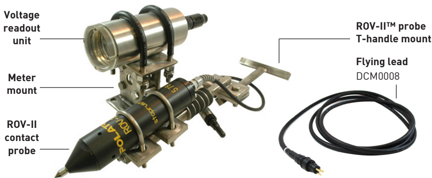
Figure 1: Deep C Meter 3000™ components
