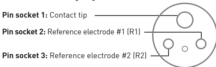
Figure 6: SEACON RMG-3FS wiring diagram
