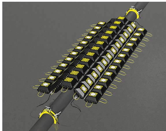
RETROCLAMPS ELECTRICALLY CONNECT THE MATS TO THE PIPELINE The mat functions both as a stabilization mattress and an anode array.
