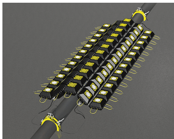
RETROCLAMPS ELECTRICALLY CONNECT THE MATS TO THE PIPELINE The mat functions both as a stabilisation mattress and an anode array.
